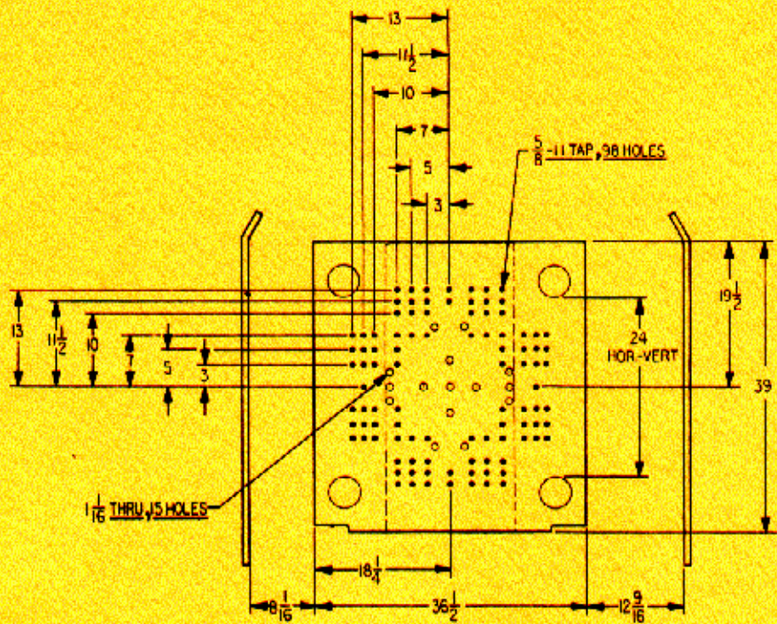
MOVABLE PLATEN
